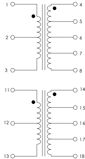
FIGURE 1: SCHEMATIC DIAGRAM
