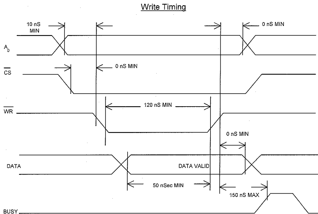
Figure 3-12 Timing Characteristics, Intel Mode
