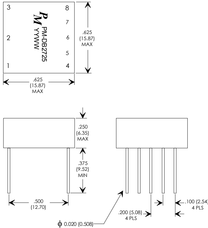
FIGURE 2: PHYSICAL DIMENSIONS IN INCHES (mm)
