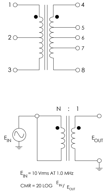
FIGURE 1: SCHEMATIC DIAGRAM
