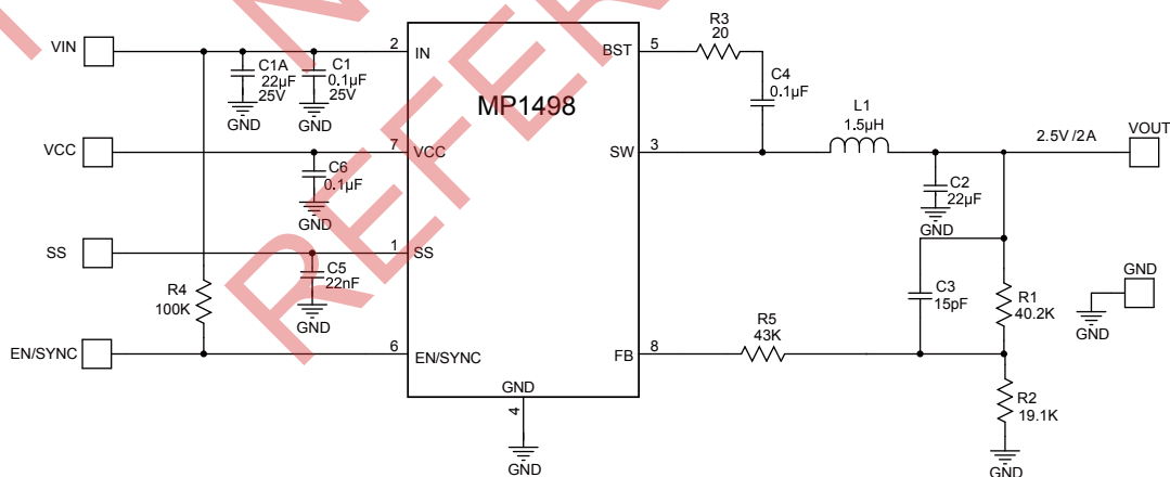
Figure 9: V_{IN}=12V , 2.5V/2A Output
