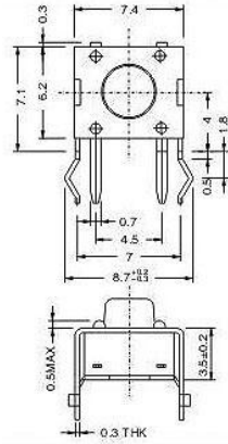
Mounting
